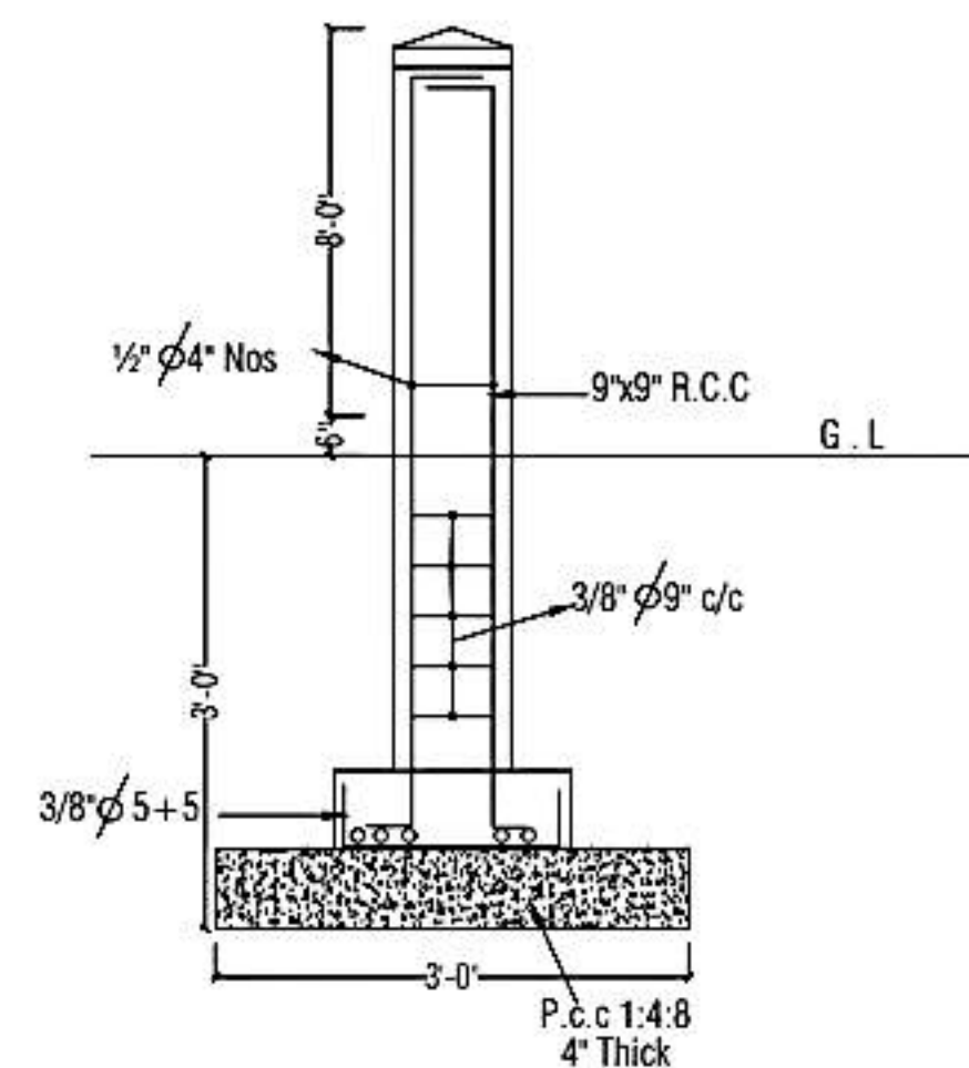
COLUMN FOUNDATION
