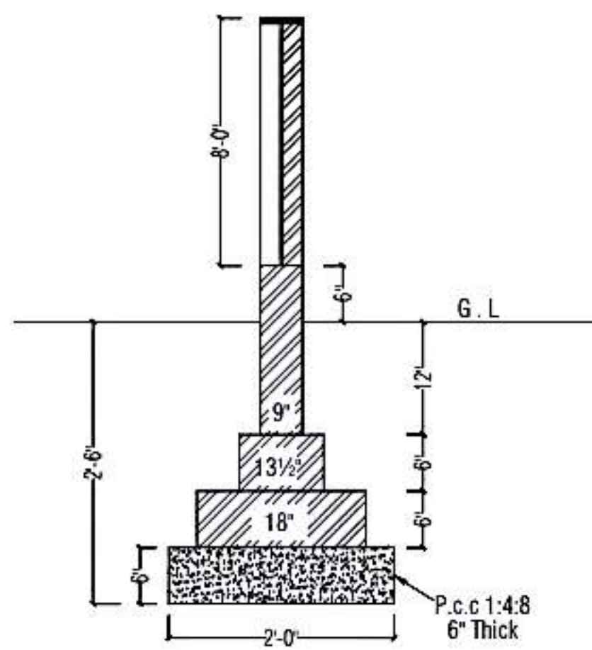
BRICK FOUNDATION
